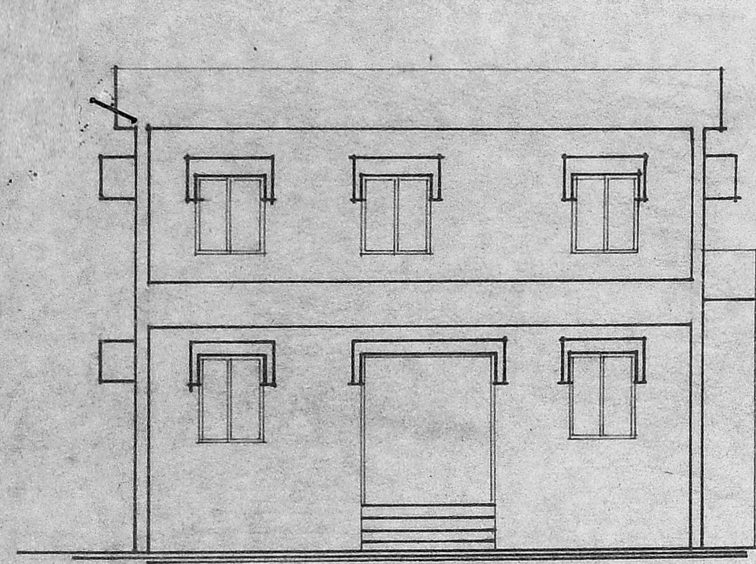
FRONT ELEVATION
